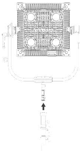
(1) To detach the yoke, first remove the fixture together with the yoke from the heavy-duty light stand and place it on a flat ground with the bottom facing up.
